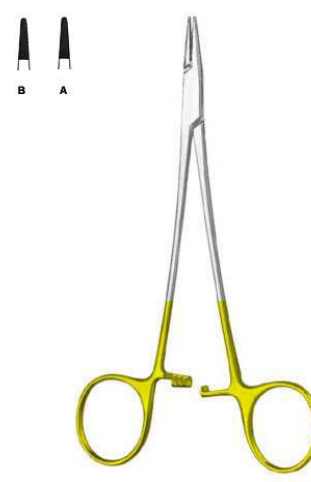
Webster DSI-4-163-13 Needle Holder with automatic release ratchet also for lefthanders Fig.233, 16 cm , 12 cm, 13cm, 15 cm
